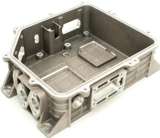
EPCU Housing
