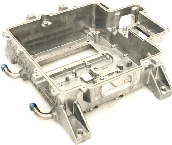
EPCU Housing
