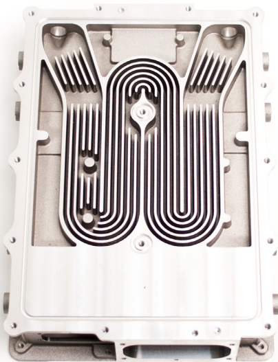
EPCU Housing
