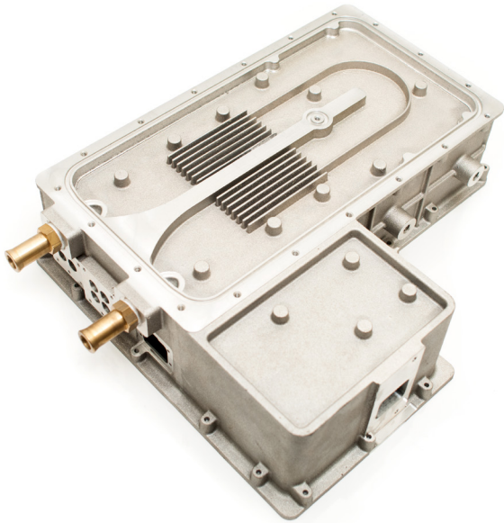
Inverter Housing (Fin Side)
